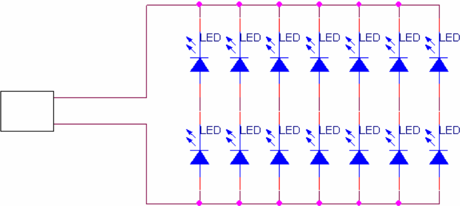
Figure 4.3 LED driver circuit
