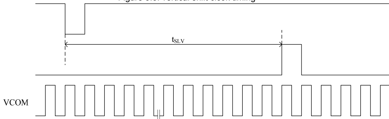
Figure 5.5: vertical shift clock timing
