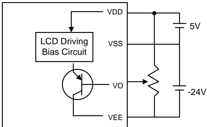
With DC/DC converter
