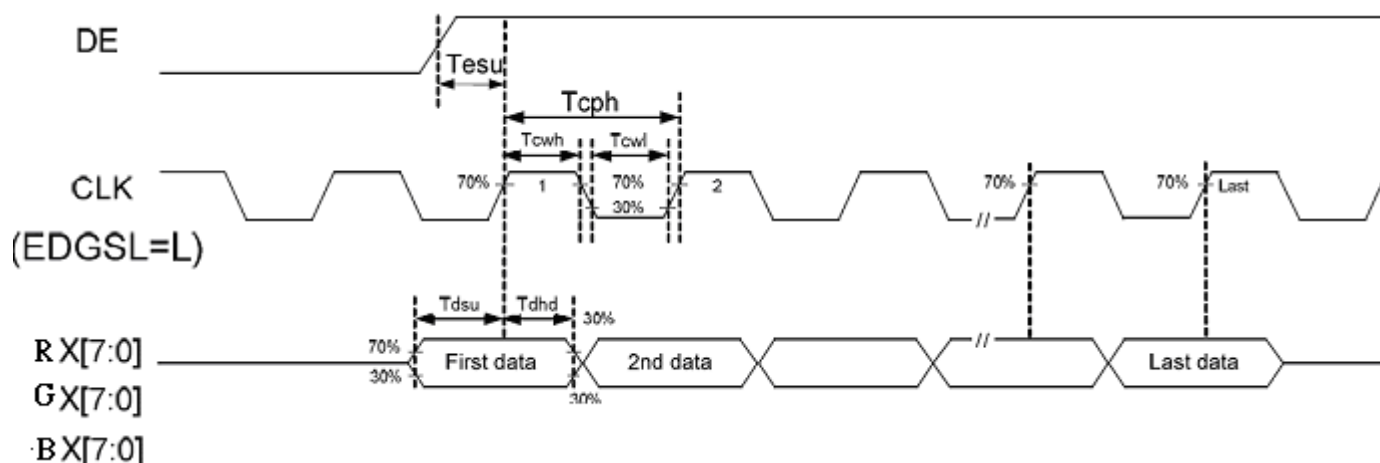
Timing Controller Timing Chart
