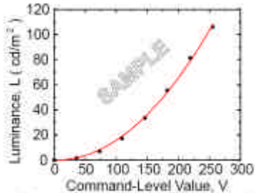
Fig. 1. Sample Luminance vs. gray scale using a 256 bit gray scale.
