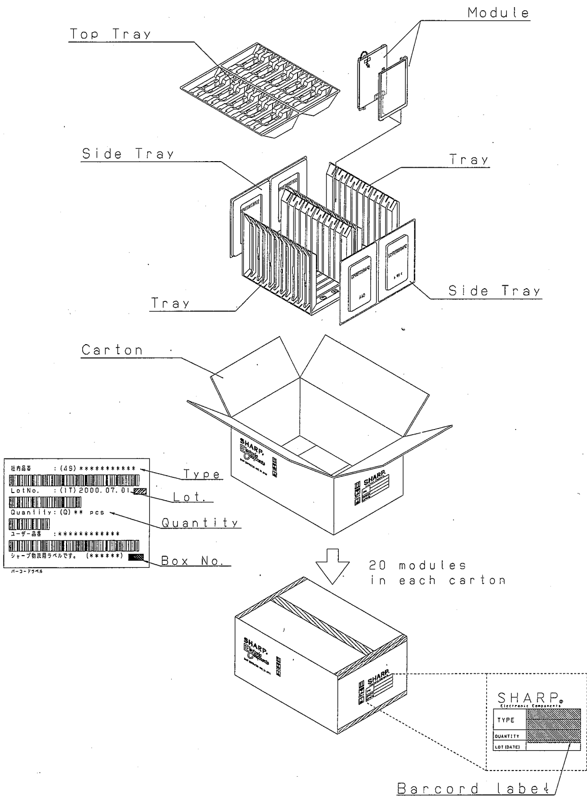
Fig 3 PACKING FORM
