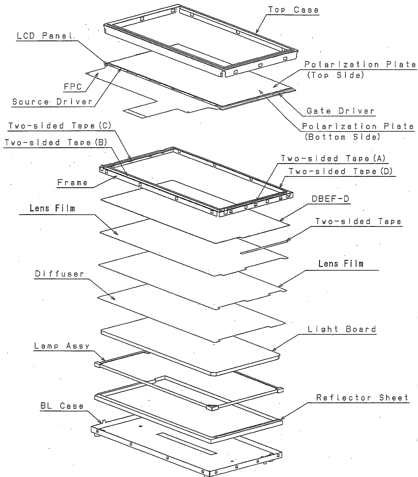
Fig.2 Assembly Diagram
