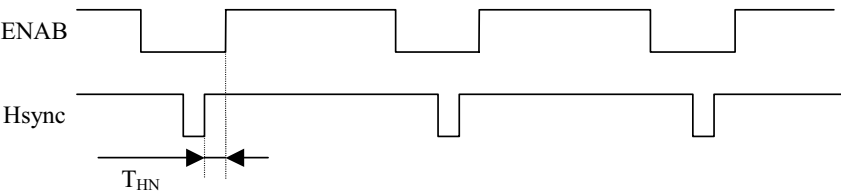
(Hsync-ENAB Phase difference)
