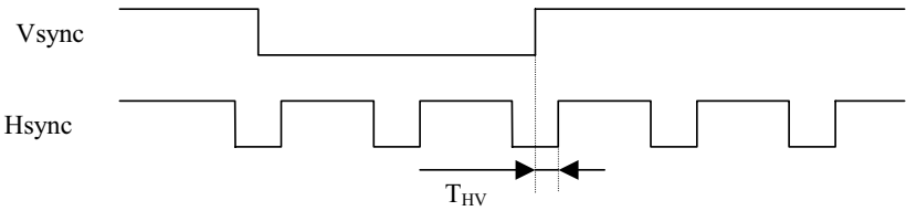
(Hsync-Vsync Phase difference)
