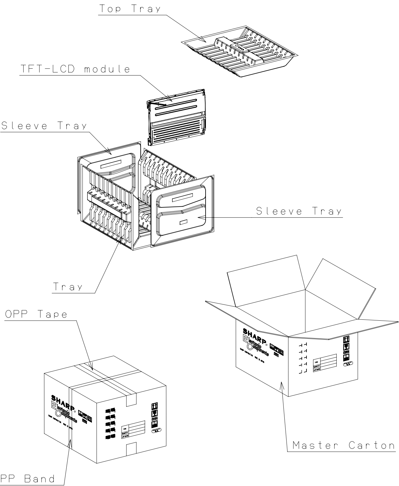
Fig4. PACKING FORM
