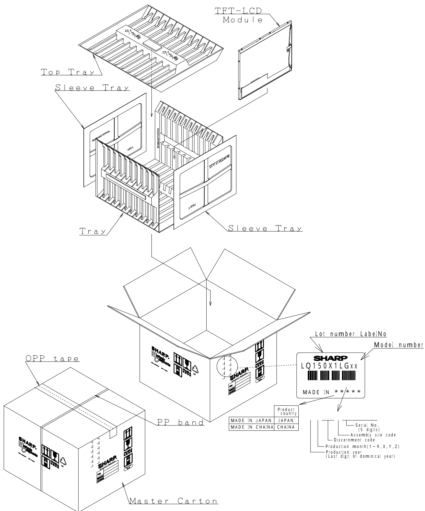
Fig3. Packing Form
