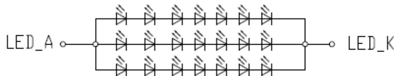
LED circuit
