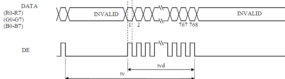
Vertical timing
