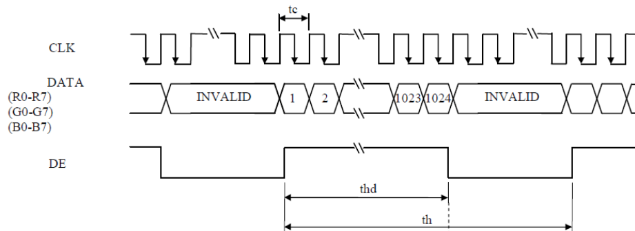
Horizontal timing
