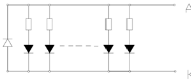
CIRCUIT DIAGRAM(1X10 LED'S)
